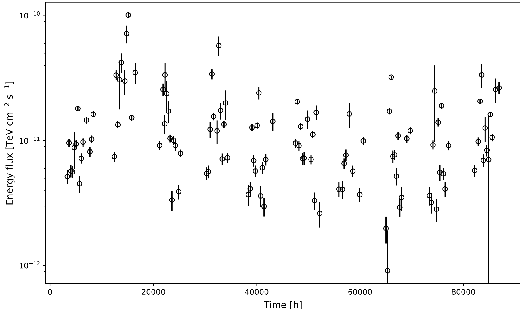
BLLac, cadence - 60 min 2 times per month - CTAO simulation
